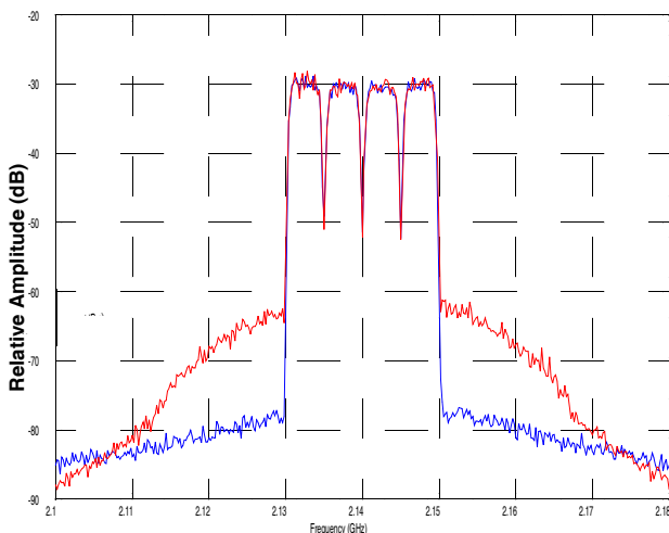
FIGURE 13. PREDISTORTION PERFORMANCE
