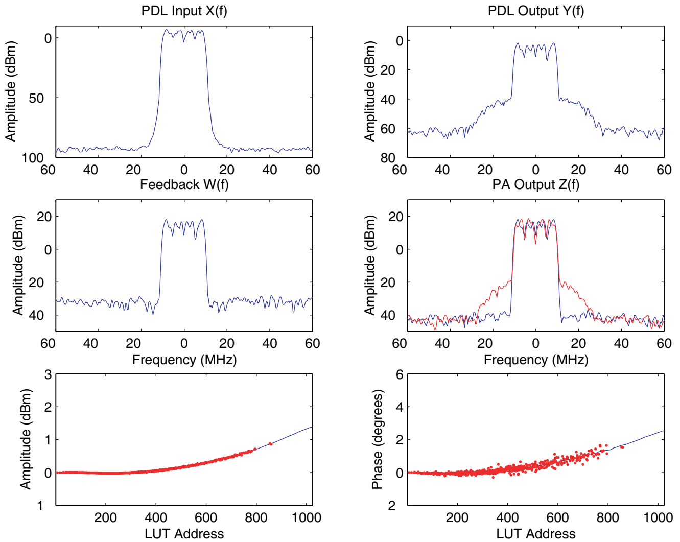
FIGURE 7. HARDWARE-IN-THE-LOOP SIMULATION
