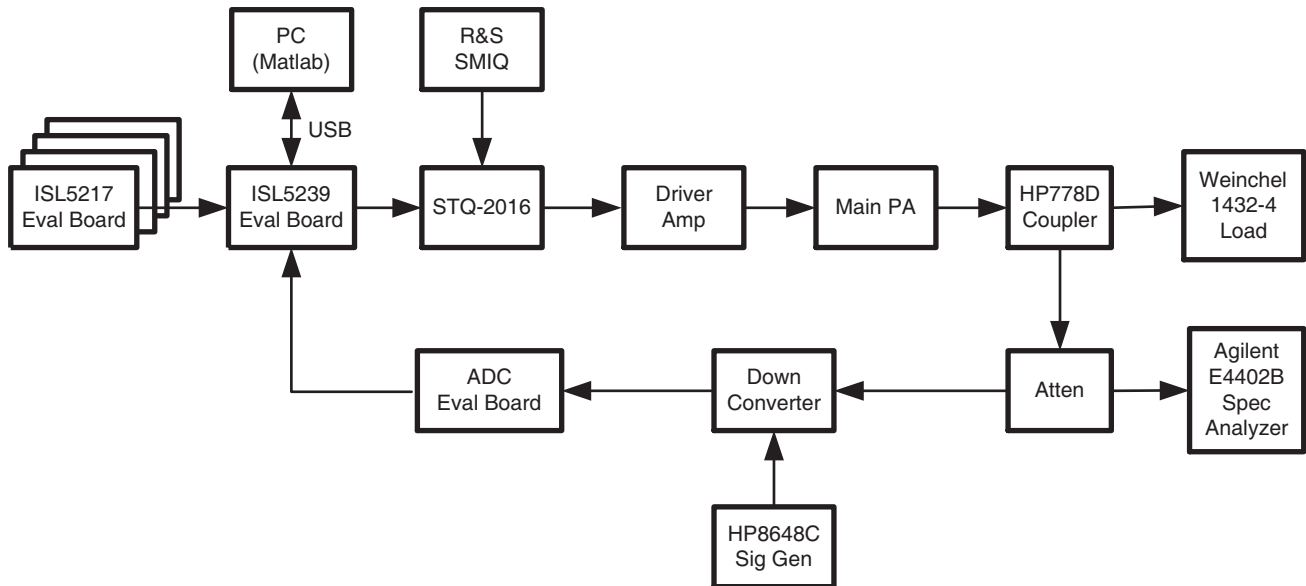
FIGURE 8. LABORATORY SETUP
